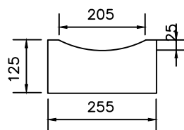
Type CD Fig NA.1h
