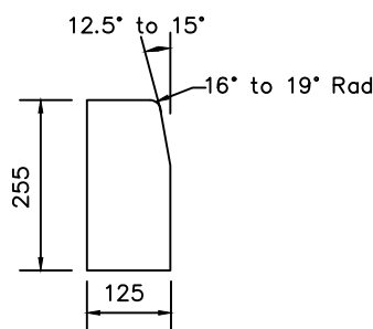
Type HB2 Fig NA.1d Half battered kerb
