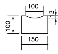
Type CD(100) (not shown in BS)
