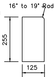
Type BN(255) Bullnosed kerb (not shown in BS)
