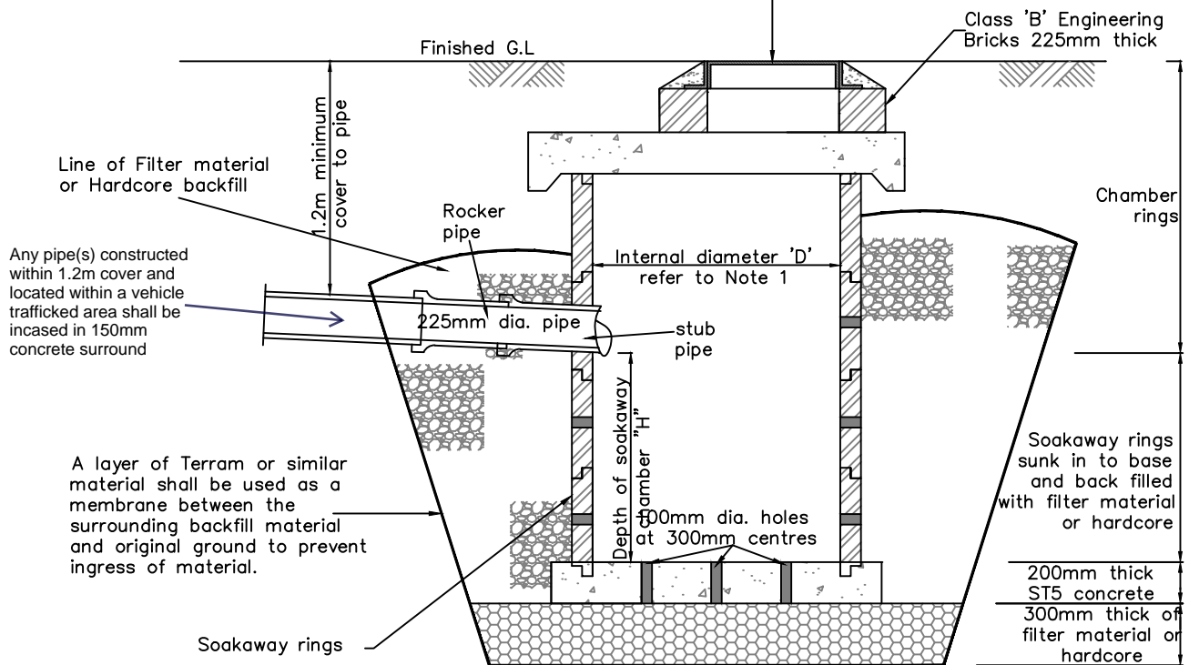
TYPICAL SOAKAWAY
