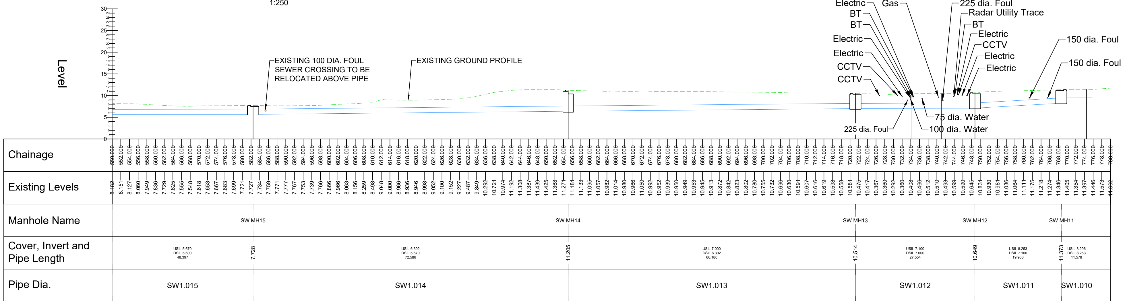
CULVERT LONG SECTION (MH15 - MH11)
